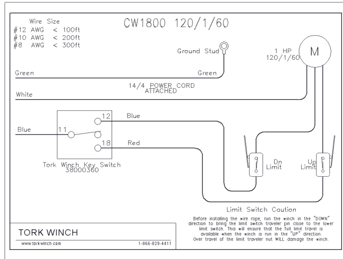
Figure 2 - Wiring 120/1/60
