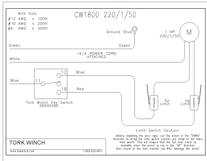
Figure 3 - Wiring 220/1/50
