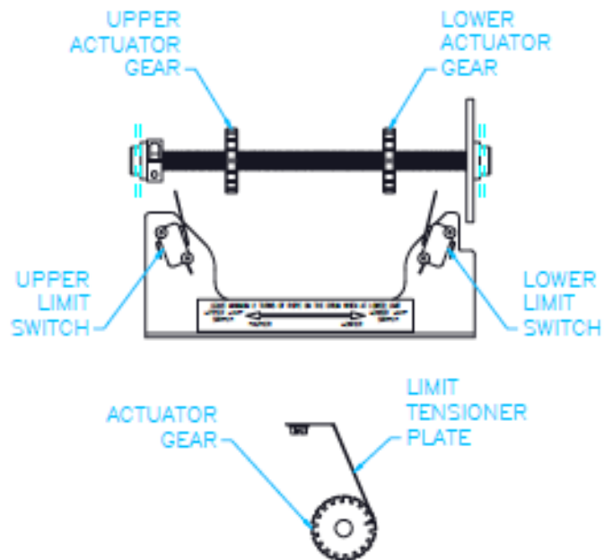
Figure 4 - Limit Switch Adjustment
