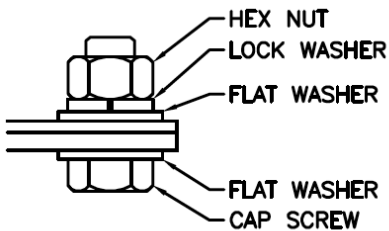
Figure 4 - Fastener Orientation
